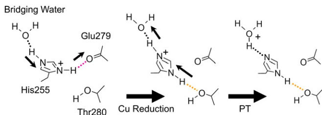
Fig. 3. Proposed mechanism of efficient PT driven by the rotation of His255. Dashed lines represent H-bonds. Strong and weak H-bonds involved in PCET are colored as in Fig. 2B. Thin black arrows illustrate the directions to which H atoms are attracted.
