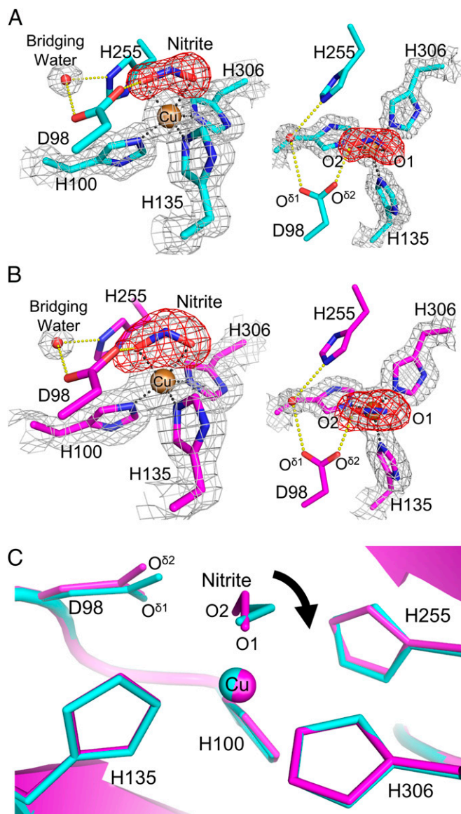
Fig. 1. NO 2 - binding in NC structures. (A) T2Cu site in the SRX NC structure (molecule A). The sigma-A-weighted 2F o -F c (1.5 \sigma ) and omit F o -F c (6.5 \sigma ) maps are shown as gray and red meshes, respectively. H-bonds (yellow) and coordination bonds (black) are represented by dashed lines. C, N, O, and Cu atoms are colored cyan, blue, red, and brown, respectively. (B) T2Cu site in the SFX NC structure (molecule A). The sigma-A-weighted 2F o -F c (1.0 \sigma ) and omit F o -F c (4.5 \sigma ) maps are shown as gray and red meshes, respectively. H-bonds and coordination bonds are represented as in A. C, N, O, and Cu atoms are colored magenta, blue, red and brown, respectively. (C) Comparison between the SFX NC (magenta) and SRX NC (cyan) structures.
